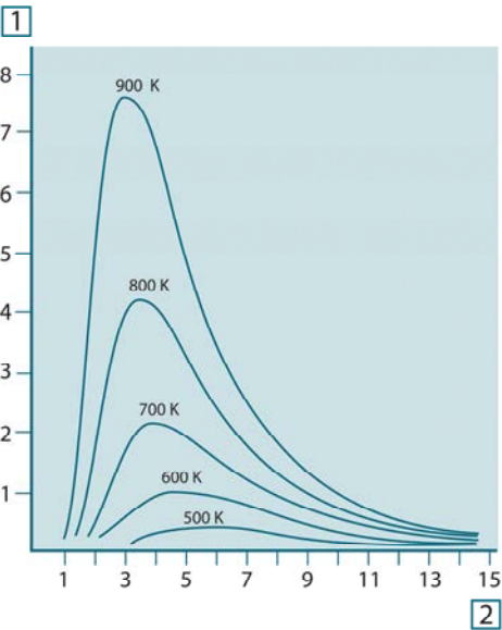
Figure 26.4 Blackbody spectral radiant emittance according to Planck's law, plotted for various absolute temperatures. 1: Spectral radiant emittance ( W/cm^2 \times 10^3(\mu m) ); 2: Wavelength ( \mu m )
